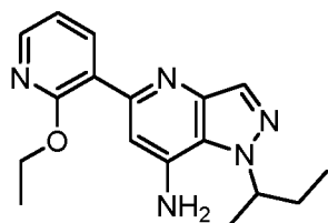
1-(sec-Butyl)-5-(2-ethoxypyridin-3-yl)-1H-pyrazolo[4,3-b]pyridin-7-amine, enantiomer 2, prepared
