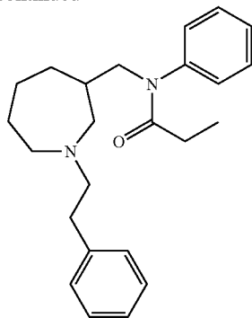
N-(1-Phenethyl-azepan-3-ylmethyl)- N-phenylpropionamide 150
