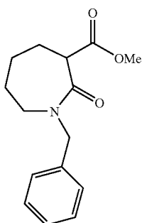
1-Benzyl-2-oxo-azepan-3-carboxylic acid methyl ester 143
