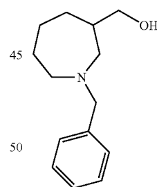
(1-Benzyl-azepan-3-yl)-methanol 144
