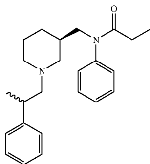
127 &amp; 128
