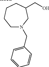
(1-Benzyl-azepan-3-yl)-methanol 144
