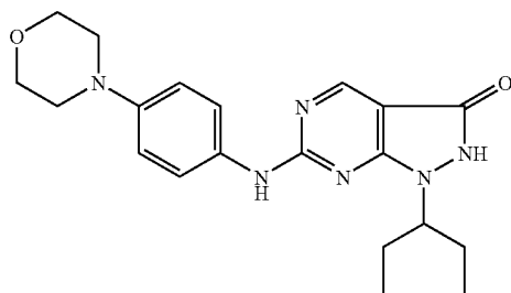
Co. No. 93; Ex. [B7]
