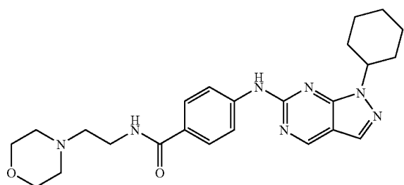
Co. No. 96; Ex. [B9]; mp. 183-185° C.
