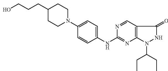
Co. No. 92; Ex. [B7]
