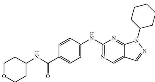
Co. No. 95; Ex. [B9]; mp. 232-233° C.
