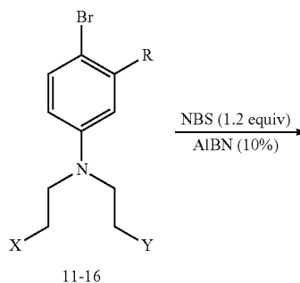
Scheme 3. Exemplary Synthesis
