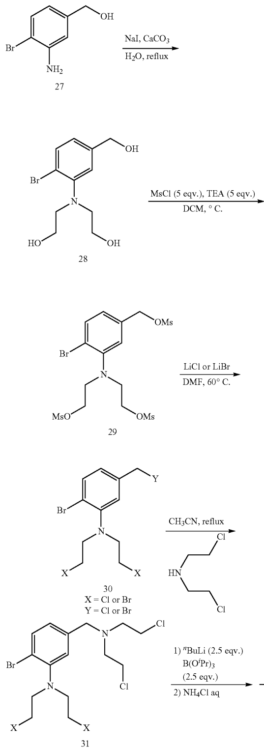
Scheme 5. Exemplary Synthesis
