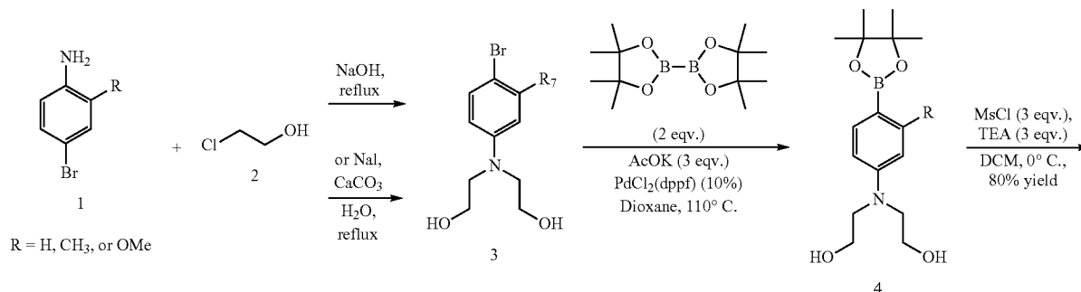
Scheme 1. Exemplary Synthesis
