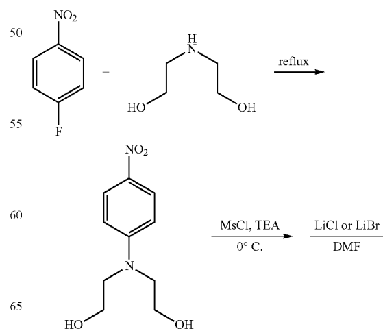
Scheme 9. Exemplary Synthesis
