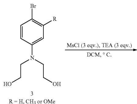
Scheme 2. Exemplary Synthesis
