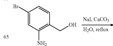
Scheme 6. Exemplary Synthesis
