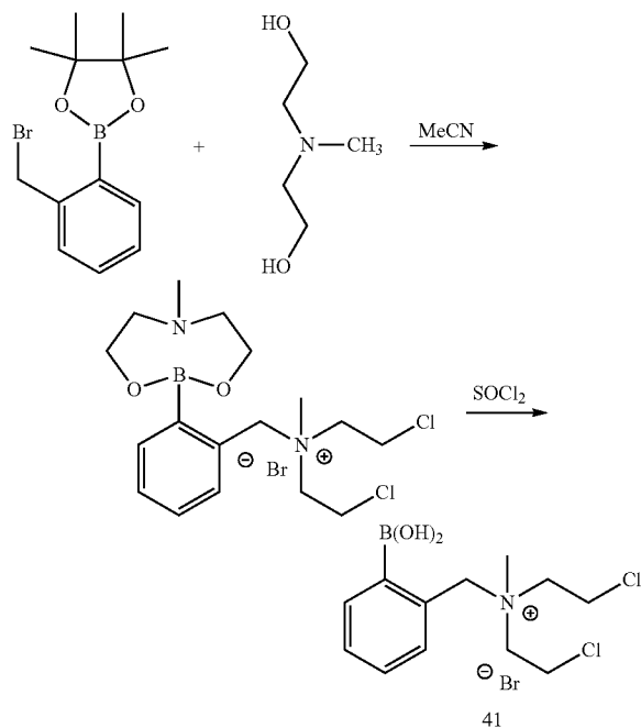
Scheme 8. Exemplary Synthesis
