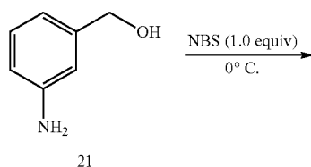
Scheme 4. Exemplary Synthesis
