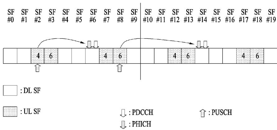
PUSCH-PHICH/UL grant timing (UL-DL configuration #1)
