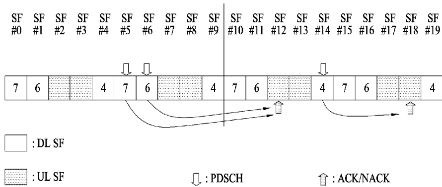
PDSCH-ACK/NACK timing (UL-DL configuration #1)
