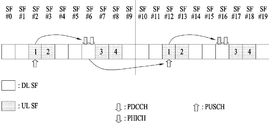
HARQ processes in UL-DL configuration #1
