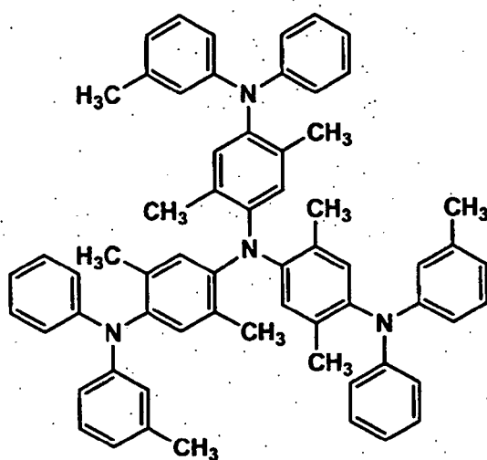
Compound 1
