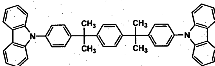
Compound 2
