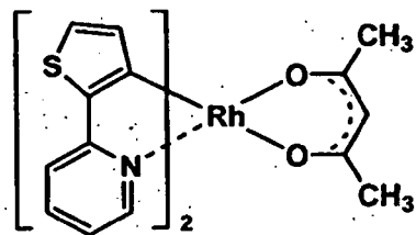
Rh-3
