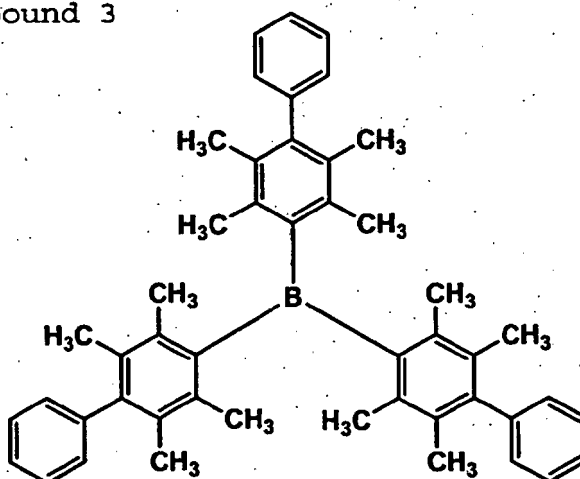
Compound 3
