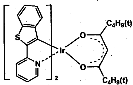
Ir-8
