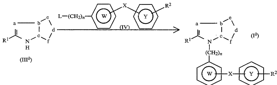
Reaction (e)
