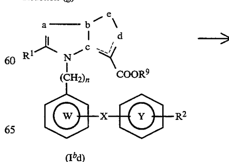
Reaction (g)
