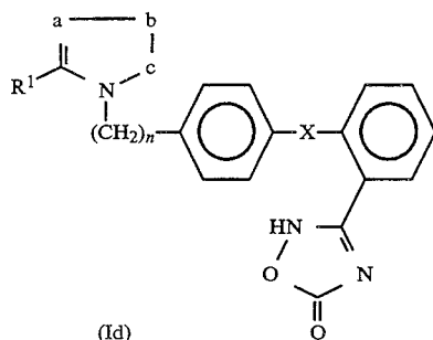
Reaction (e)
