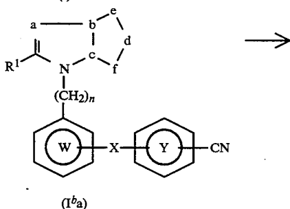
Reaction (f)
