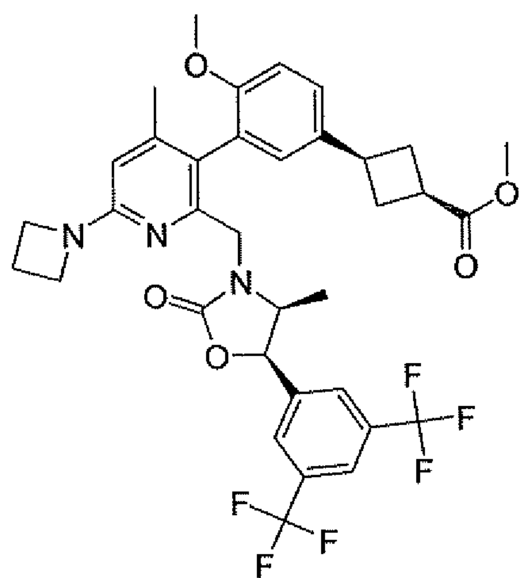
Atropisomers A and B
