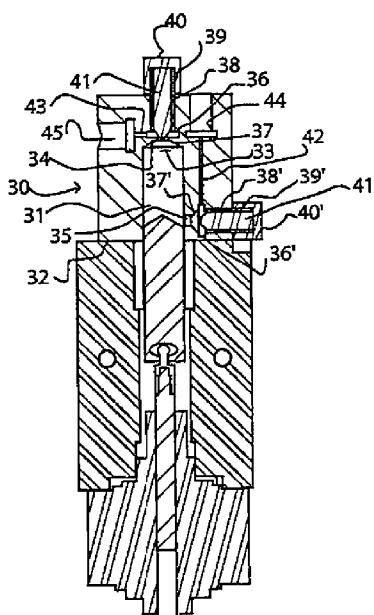
CROSS-SECTION A-A
