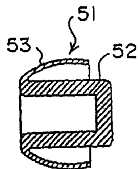
FIG. 6 (PRIOR ART)
