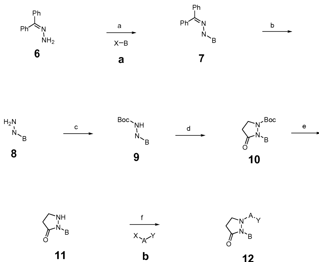
Scheme 2
