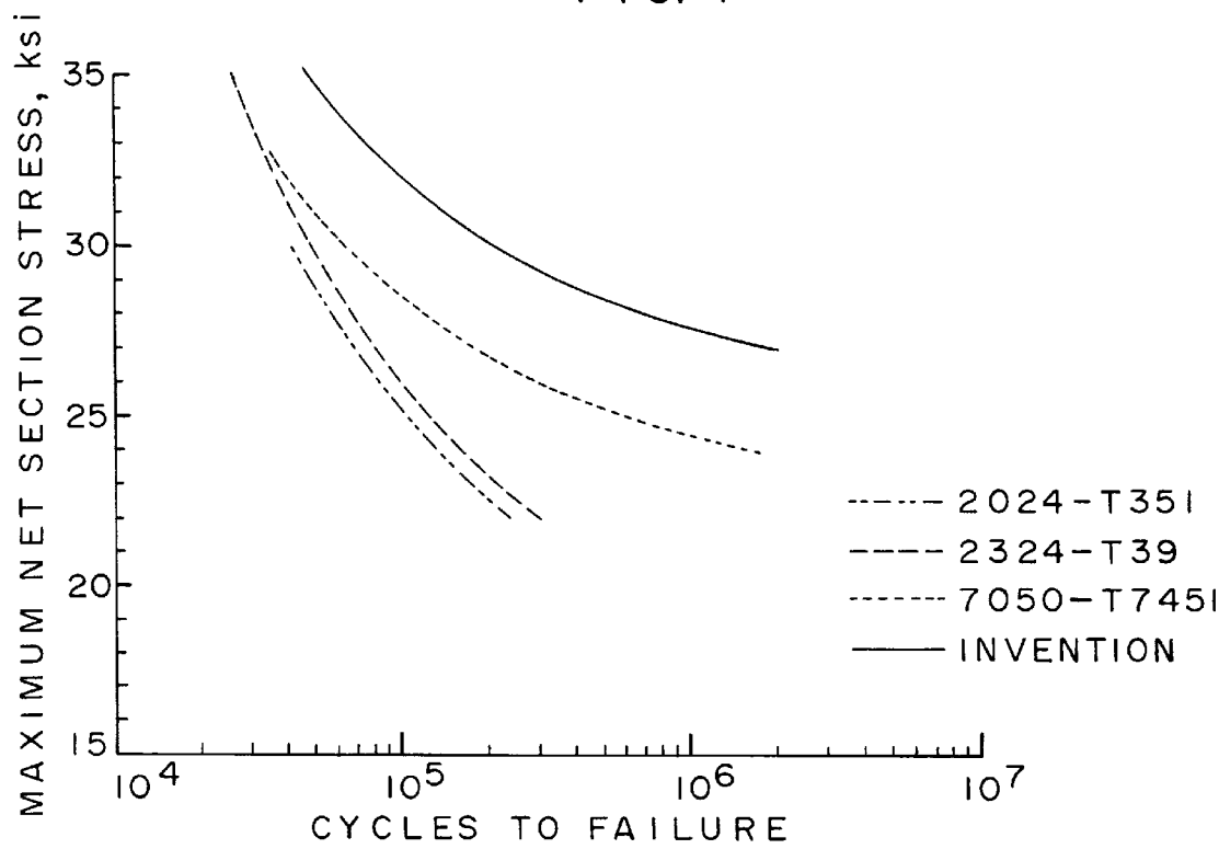
S/N FATIGUE COMPARISON
