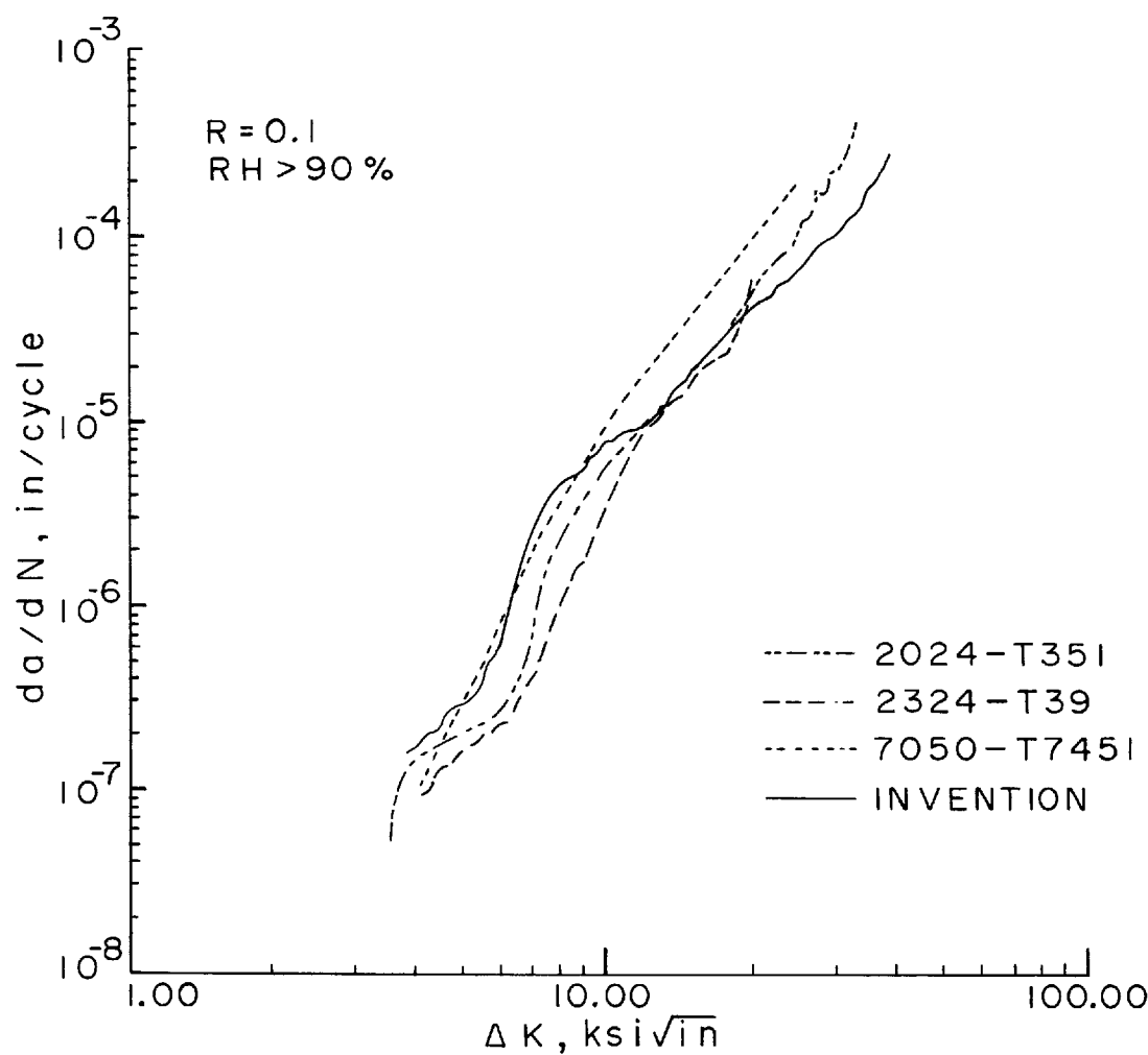
FATIGUE CRACK GROWTH COMPARISON
