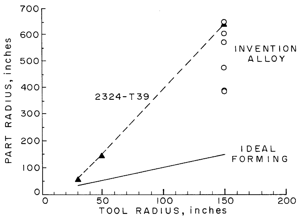
AGE FORMING RESPONSE
