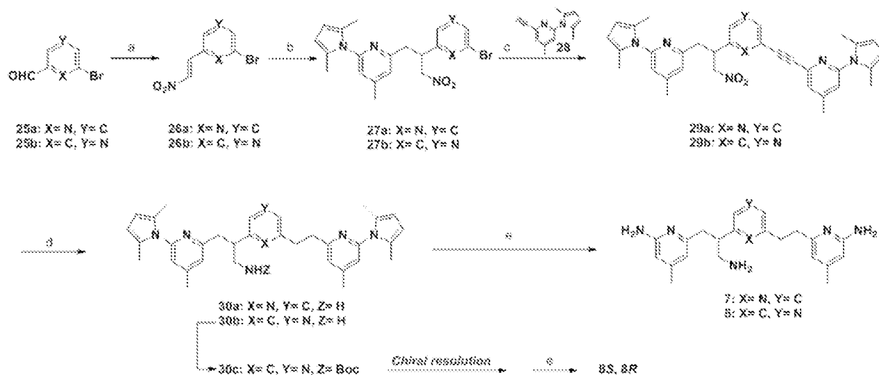
Scheme 18. Synthesis of 7 and 8
