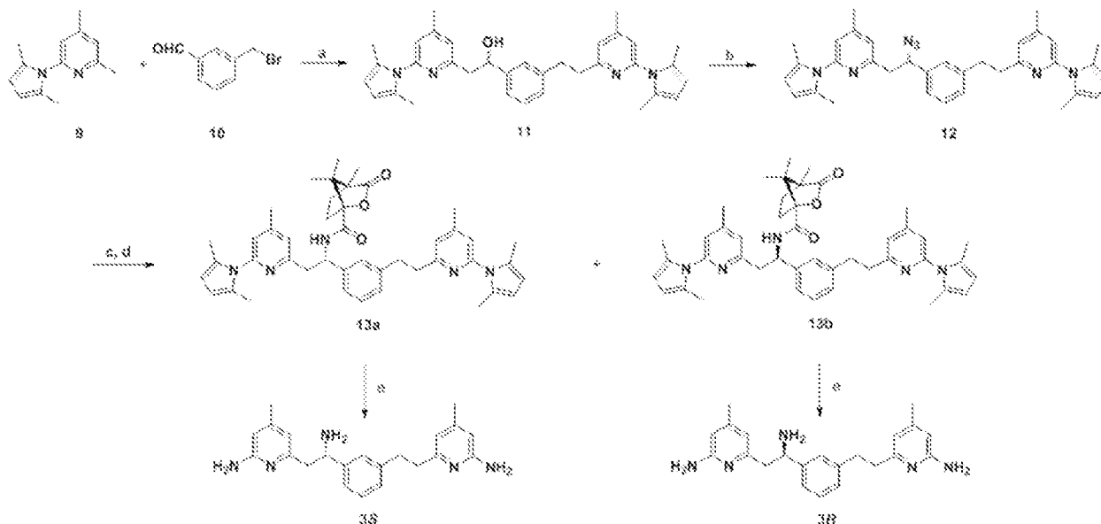
Scheme 15. Synthesis of 3R and 3S. a
