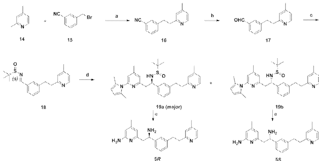
Scheme 16. Synthesis of 5 R and 5 S . a
