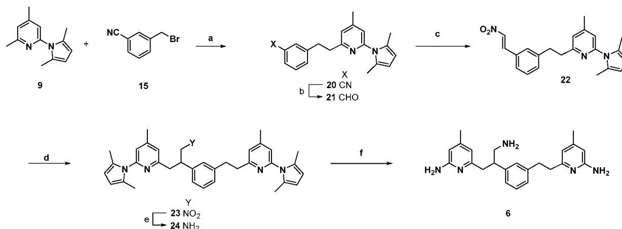
Scheme 17. Synthesis of 5
