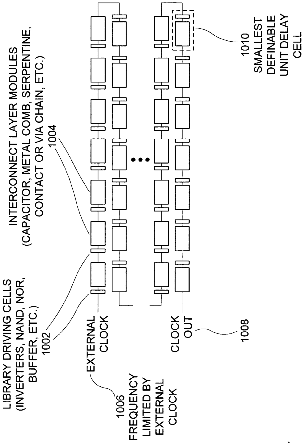
1000 CHAIN OF UNIT DELAY CELLS USING AN EXTERNAL CLOCK AS THE IO DATA INPUT
