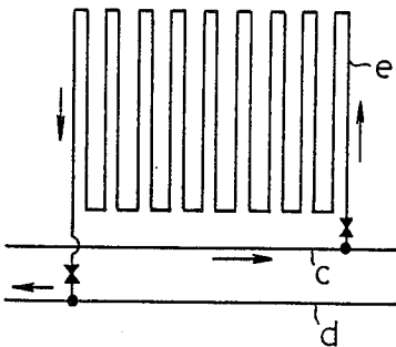
FIG. 20B (PRIOR ART)
