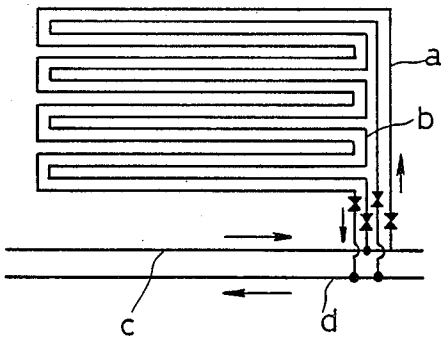
FIG. 20A (PRIOR ART)
