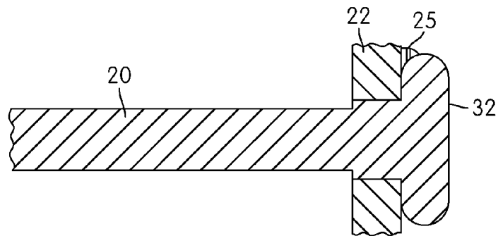
FIG. 5 (PRIOR ART)
