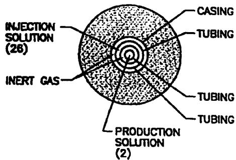
FIGURE 3C CROSS SECTION DETAIL A-A'
