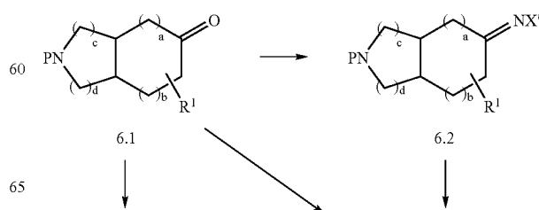
Scheme 6
