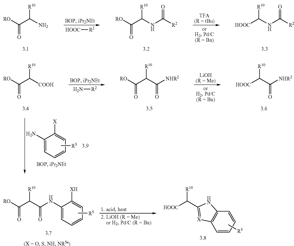
Scheme 3.
