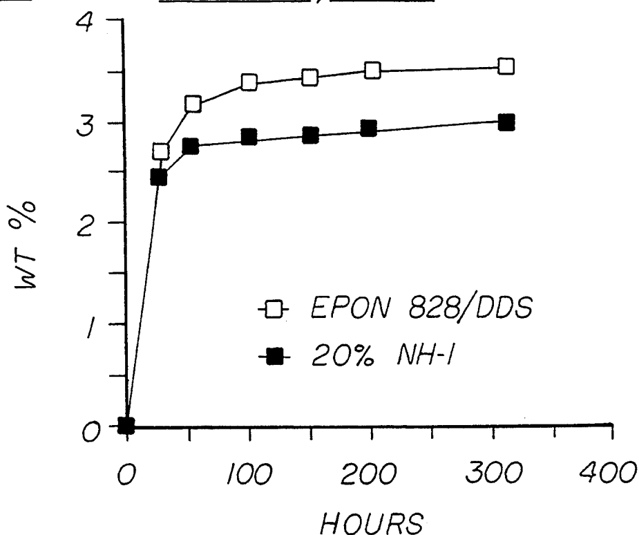
Fig. 4 PERCENT WATER ABSORBED BY EPON 828/DDS
