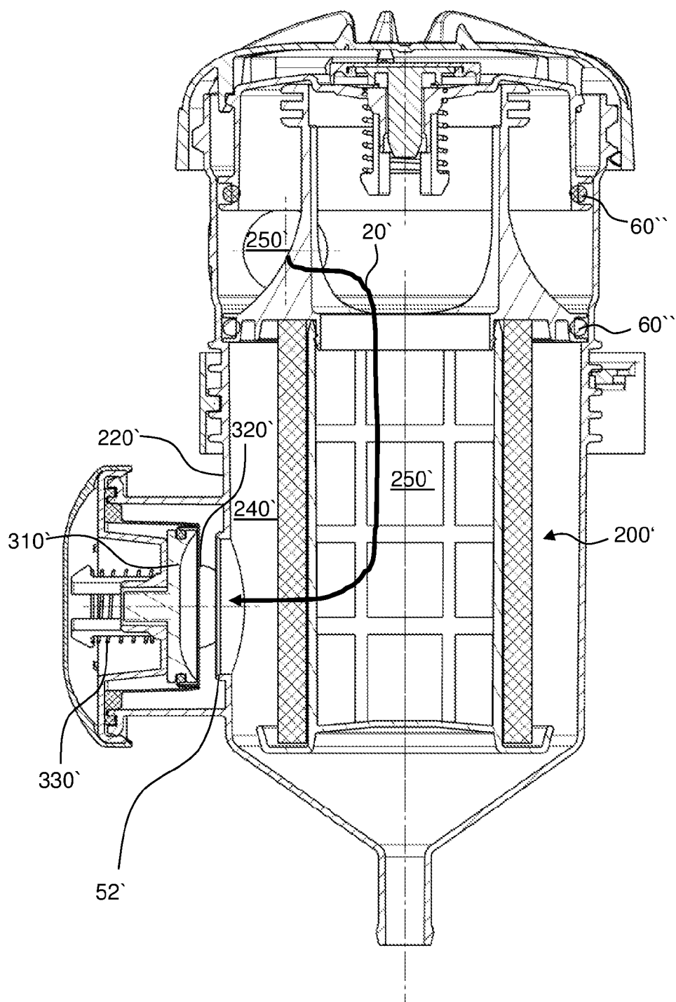
Fig. 12 Prior Art
