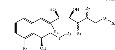
Formula (IX)
