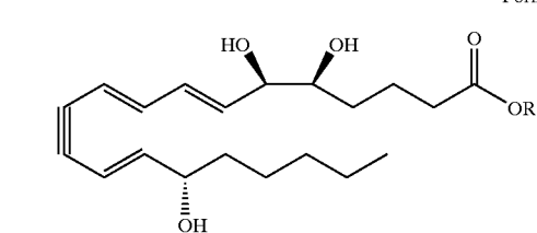
Formula (XI)
