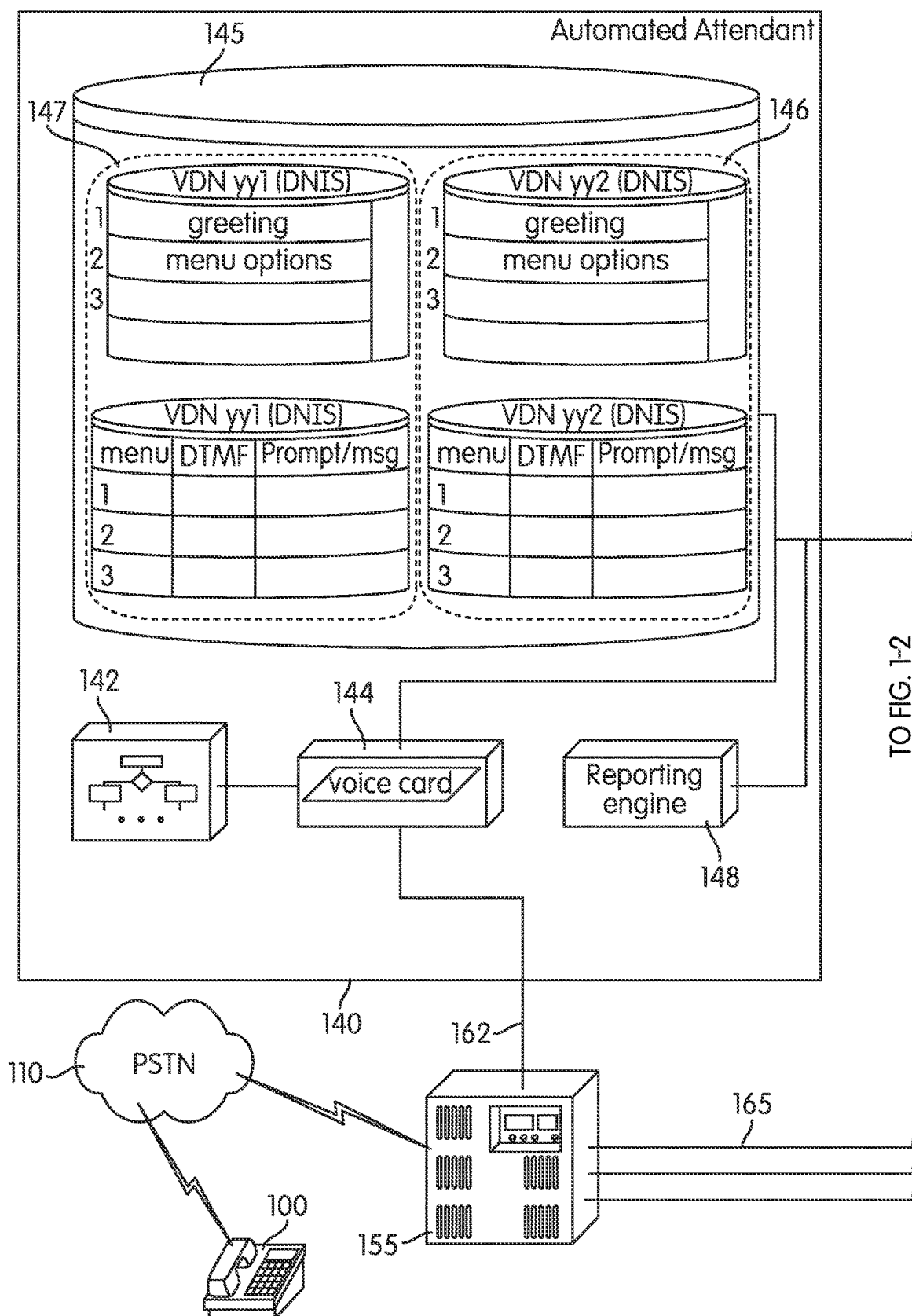
FIG. 1-1 PRIOR ART
