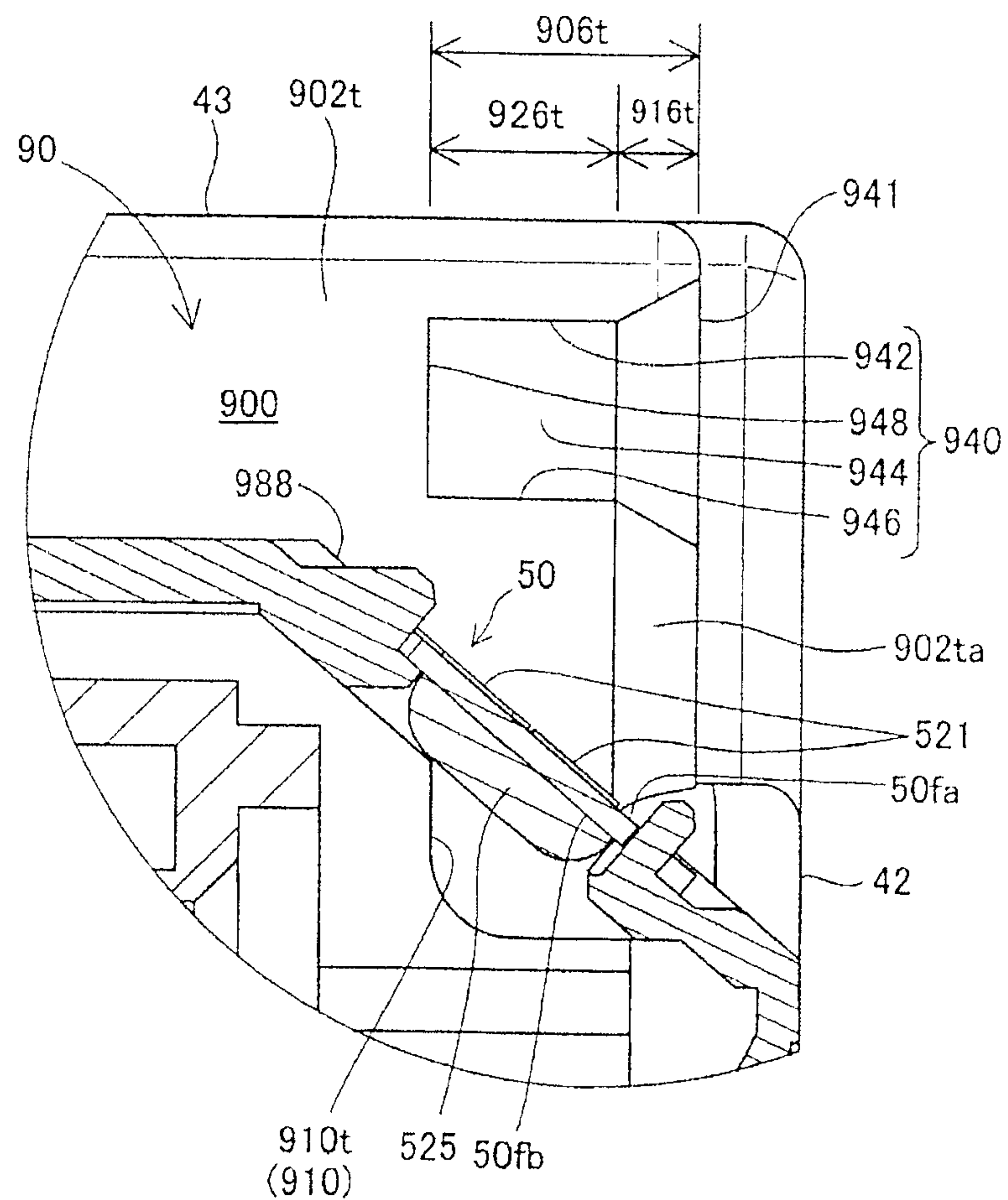
28b-28b CROSS-SECTIONAL VIEW
