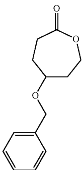
5-(Benzyloxymethyl)oxepan-2-one (BOMXO)
