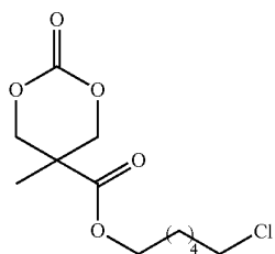
(MTC-C6Cl)
