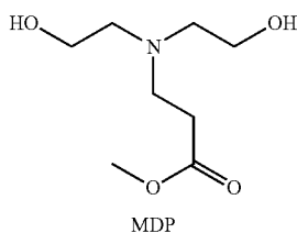
Example 20. Preparation of Diol MDP
