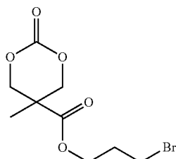
(MTC-PrBr)
