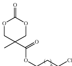
(MTC-C8Cl)
