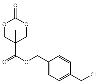
(MTC-BnCl)
