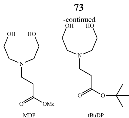
Example 20. Preparation of Diol MDP
