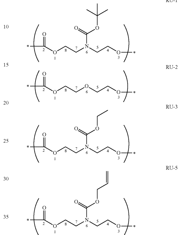
Scheme 3.
