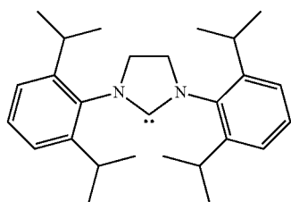
1,3-Bis(2,6-di-i-propylphenyl)-4,5-dihydroimidazol-2-ylidene (Im-8)
