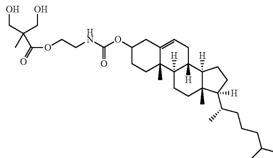
(Chol-MPA)
