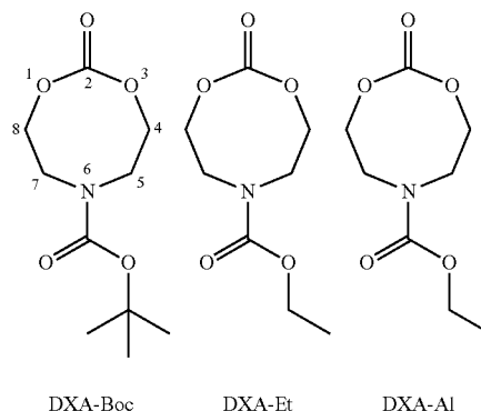
Scheme 2.
