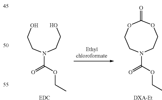
Example 23. Preparation of Ethyl 2-Oxo-1,3,6-Dioxazocane-6-Carboxylate (DXA-Et)
