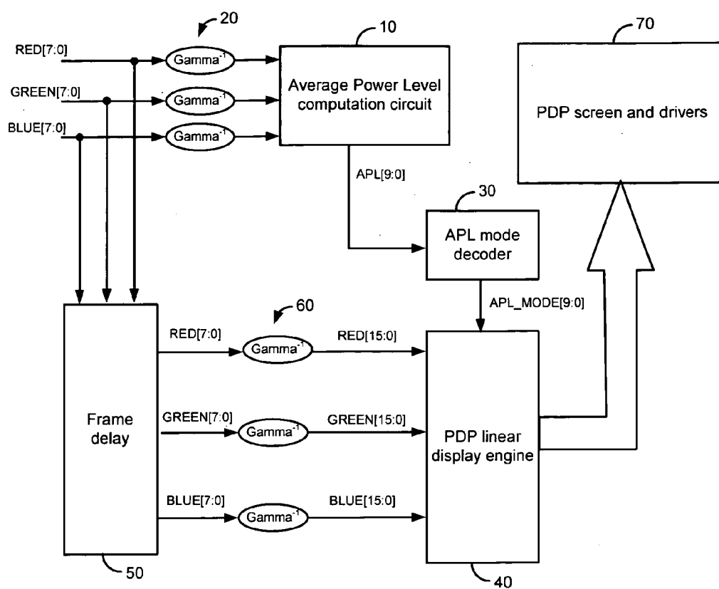
FIG.1 (PRIOR ART)
