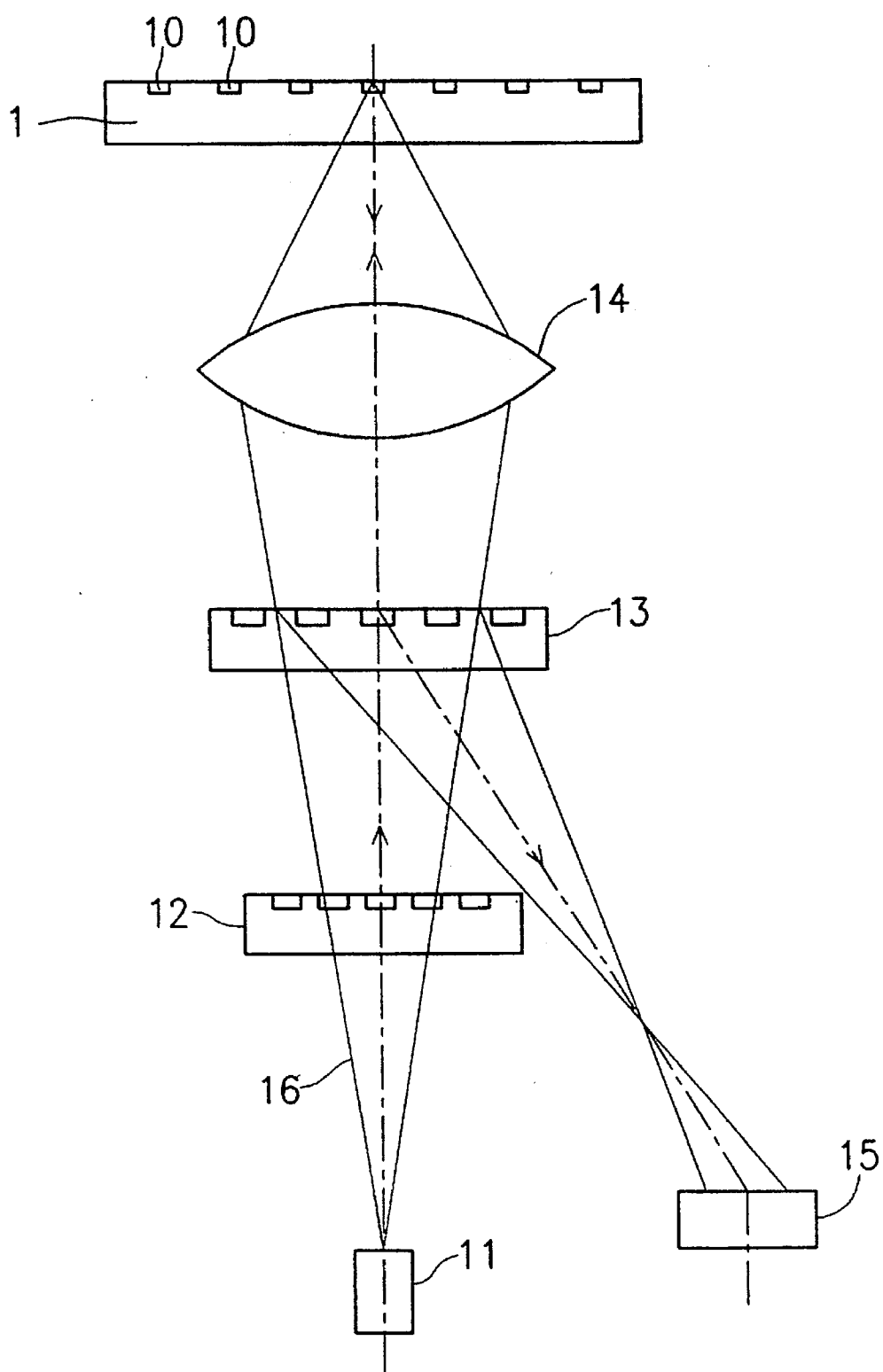
FIG. 1 (PRIOR ART)
