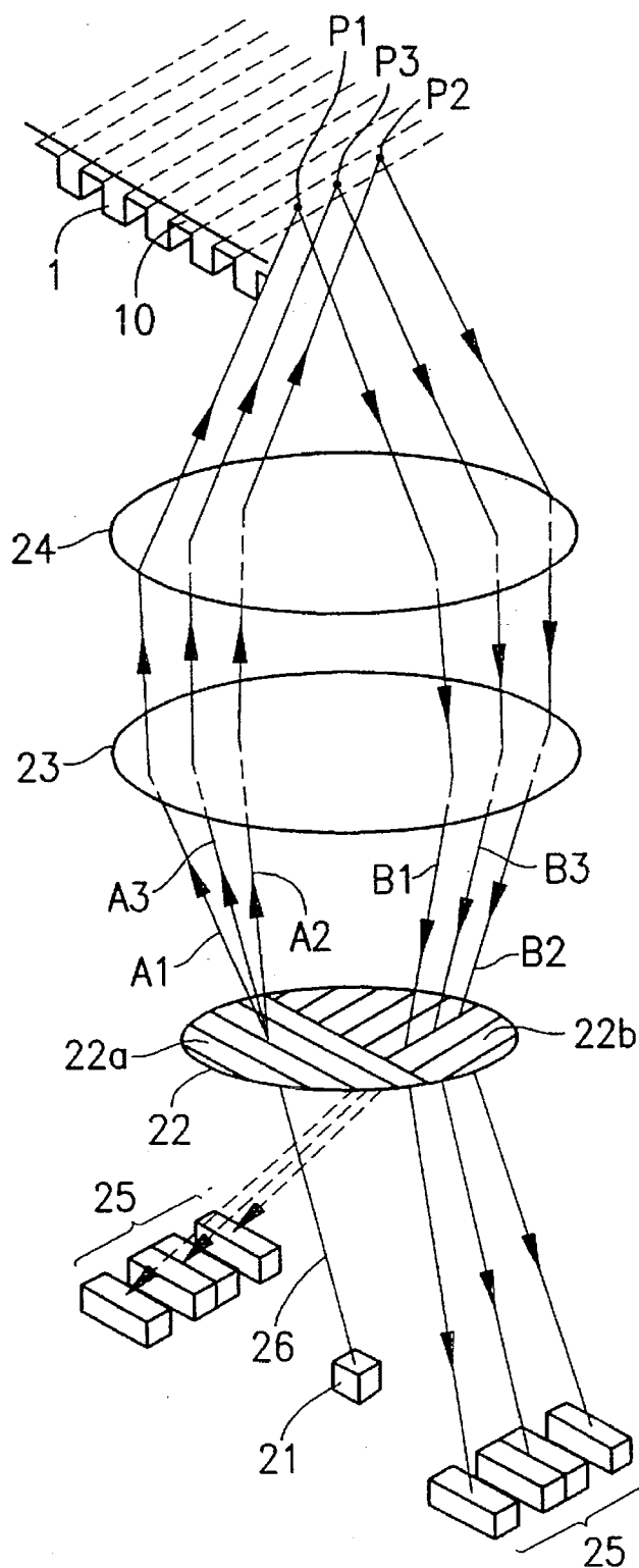
FIG. 2 (PRIOR ART)
