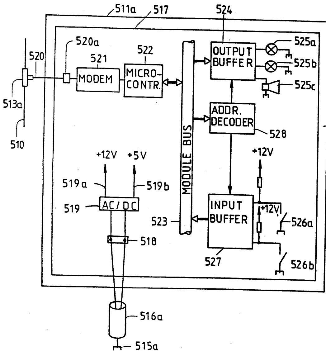
FIG. 13 INTELLIGENT ROOM BOX
