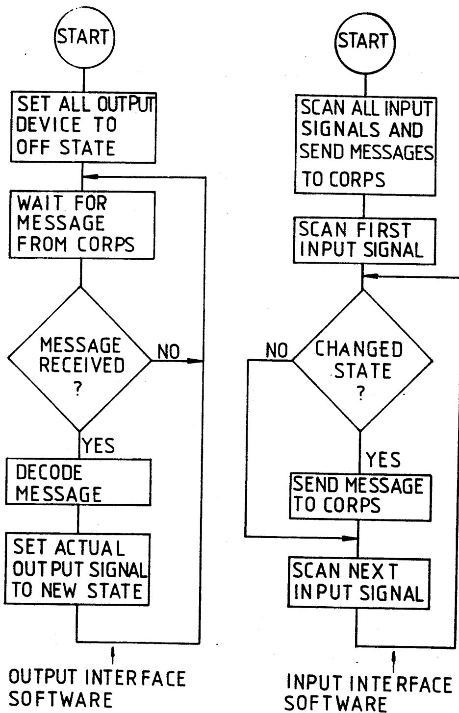
FIG. 14 SOFTWARE FLOW DIAGRAM
