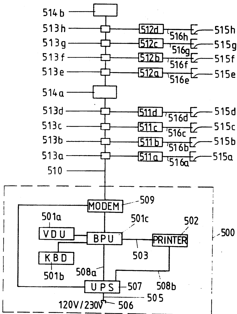
FIG. 12 EMBODIMENT WITH BROADBAND CABLE
