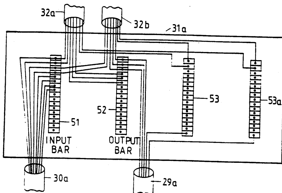
FIG. 4 JUNCTION BOX
