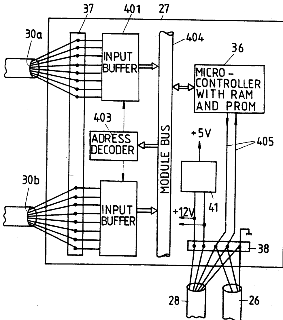
FIG. 2 INPUT INTERFACE CARD
