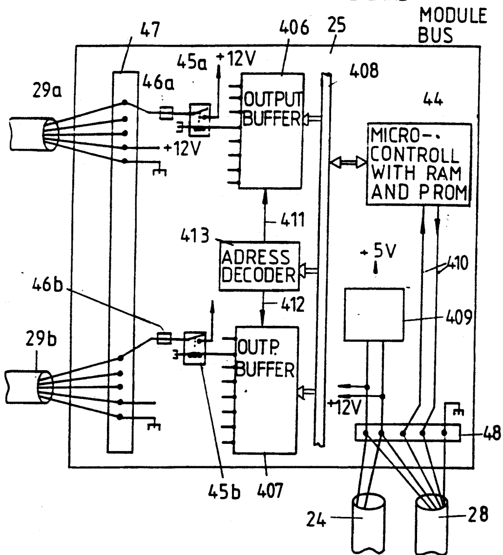
FIG. 3 OUTPUT INTERFACE CARD
