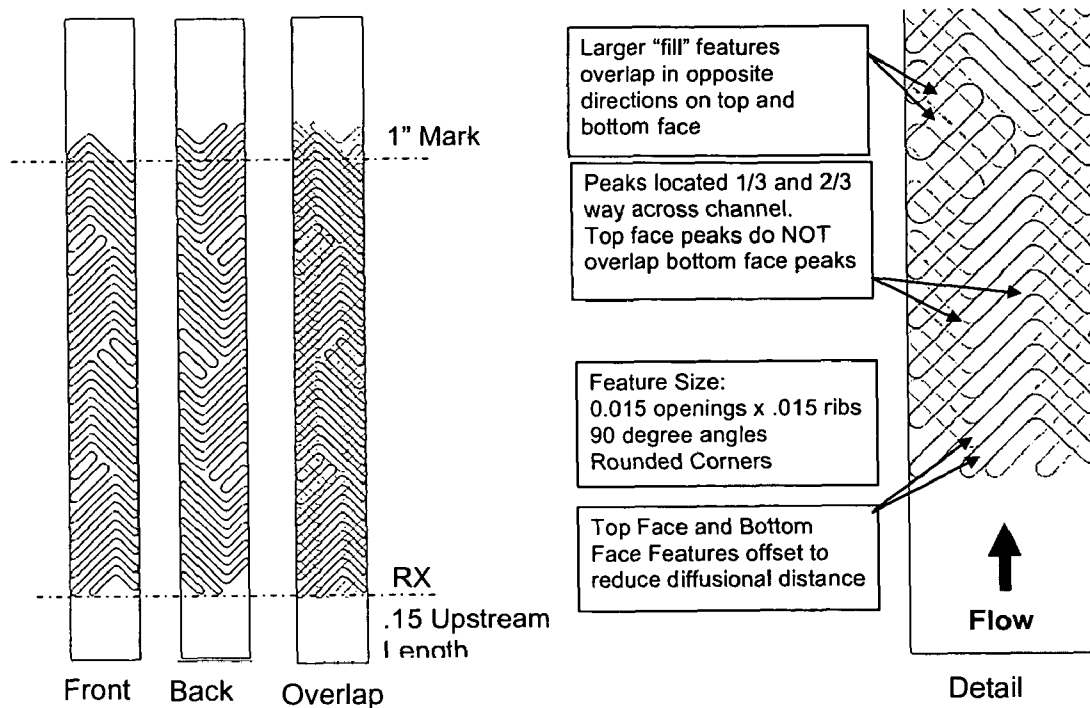
Figure 3. Concept A design detail
