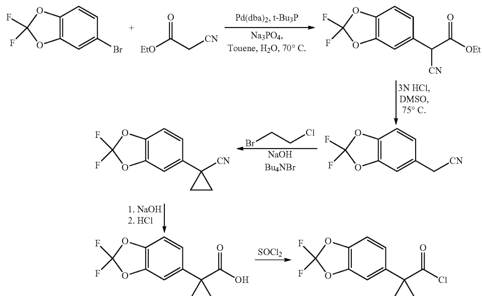
Scheme 2. Alternative synthesis of the acid chloride moiety.
