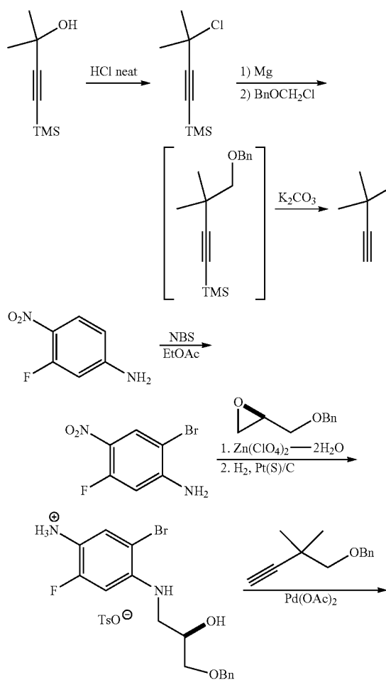
Scheme 3. Synthesis of the amine moiety.
