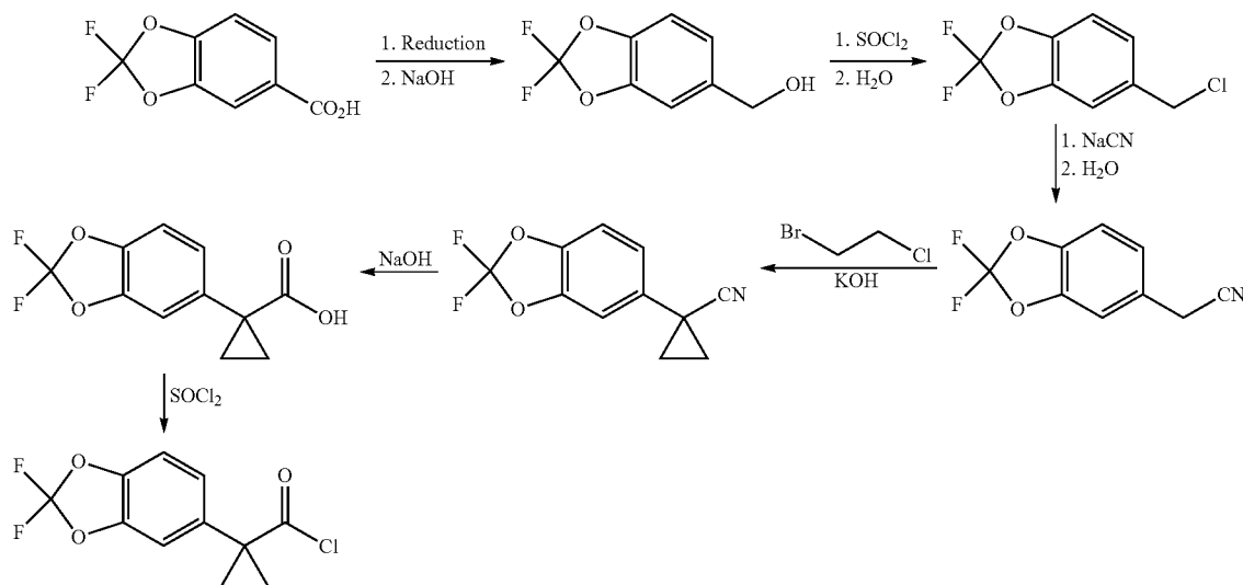
Scheme 1. Synthesis of the acid chloride moiety.
