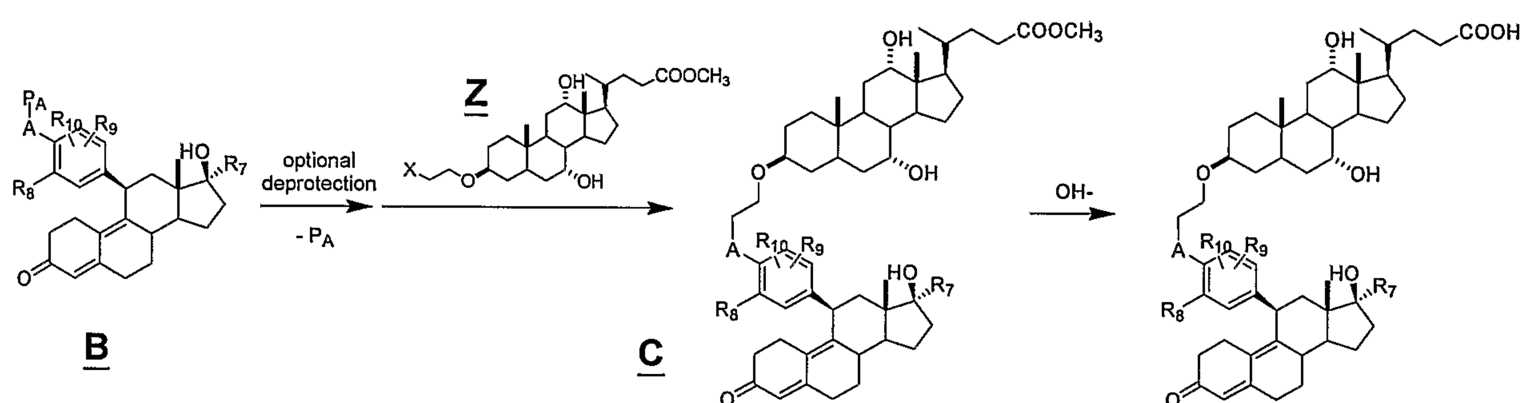
Scheme 3. Assembly of fragments
