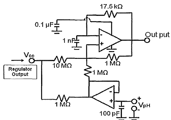
Figure 20 The relaxation oscillator design in the transponder.
