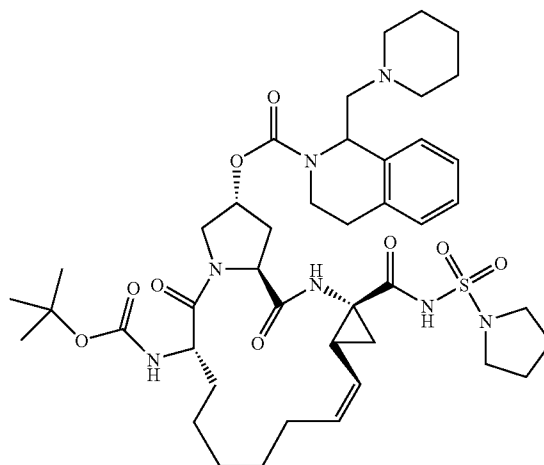
Compound 109
