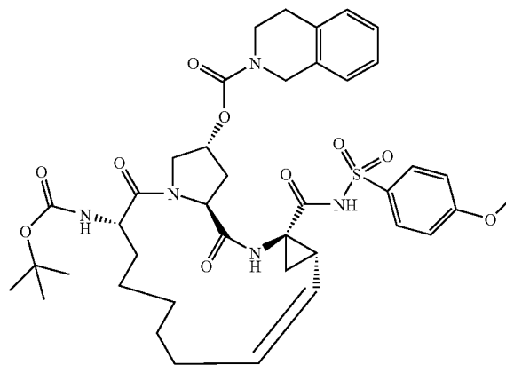
Compound AR00320548
