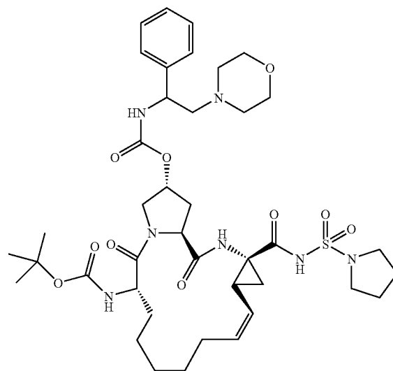
Compound 112
