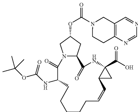
Compound AR00304183
