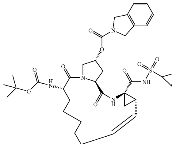
Compound AR00294381
