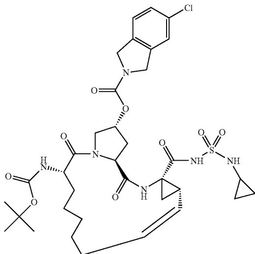
Compound 114
