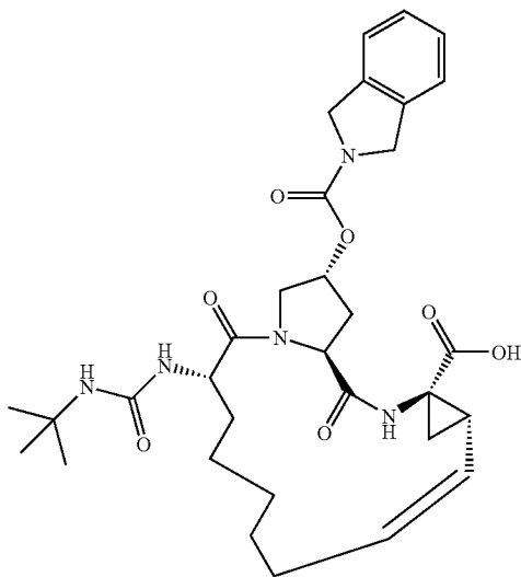
Compound AR00320078
