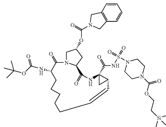
Compound 119
