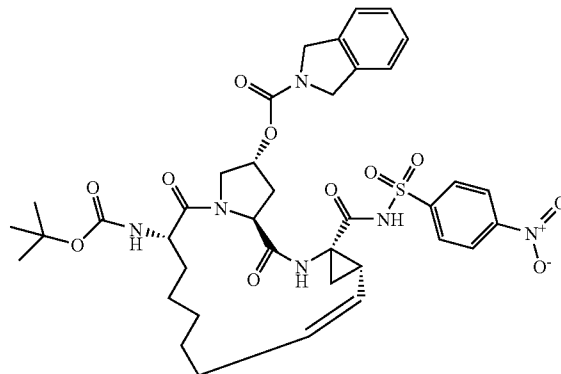
Compound AR00334249
