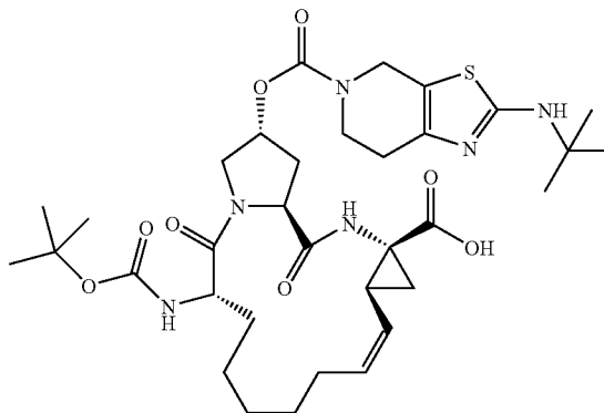
Compound AR00304103
