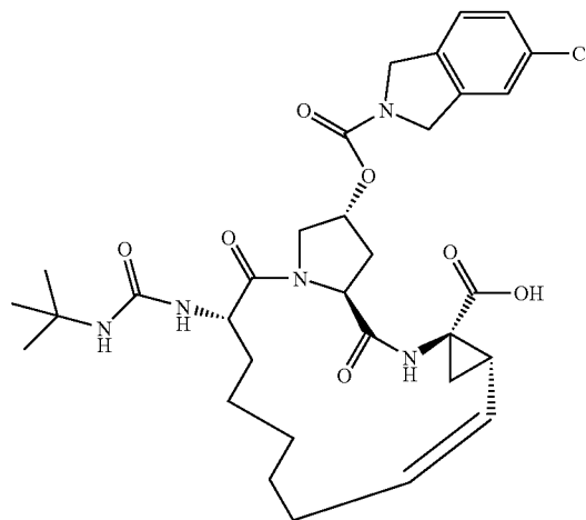
Compound AR00320449
