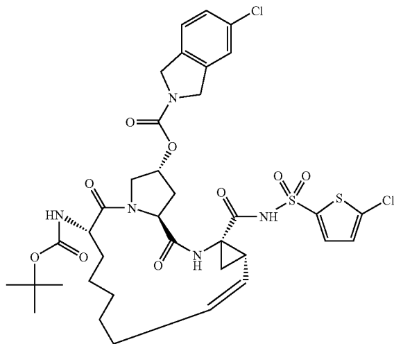
Compound AR00340173
