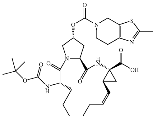
Compound AR00304158
