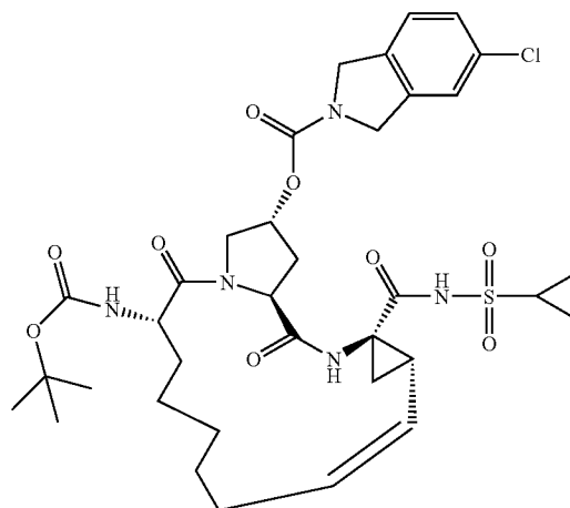
Compound AR00320119
