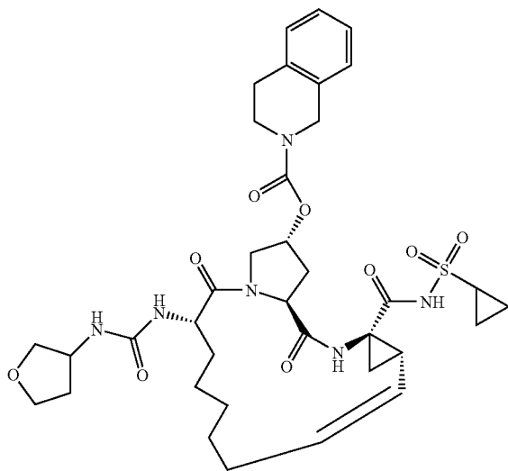
Compound AR00320222
