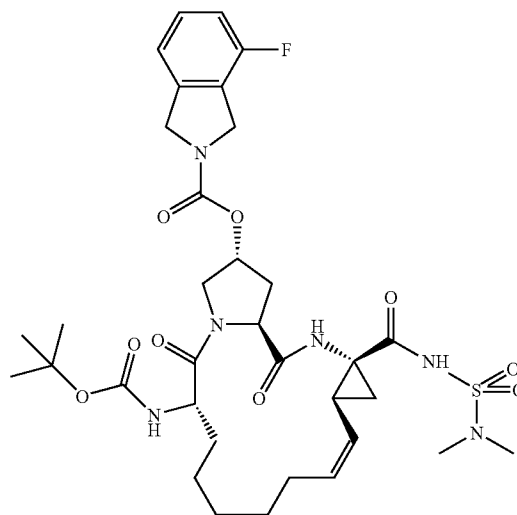
Compound 106
