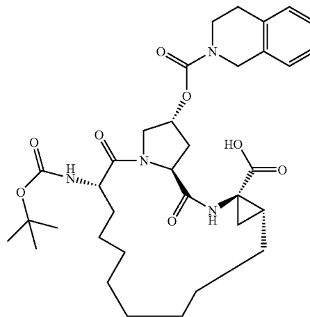
Compound AR00312023
