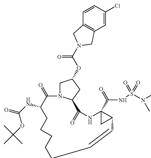
Compound 113
