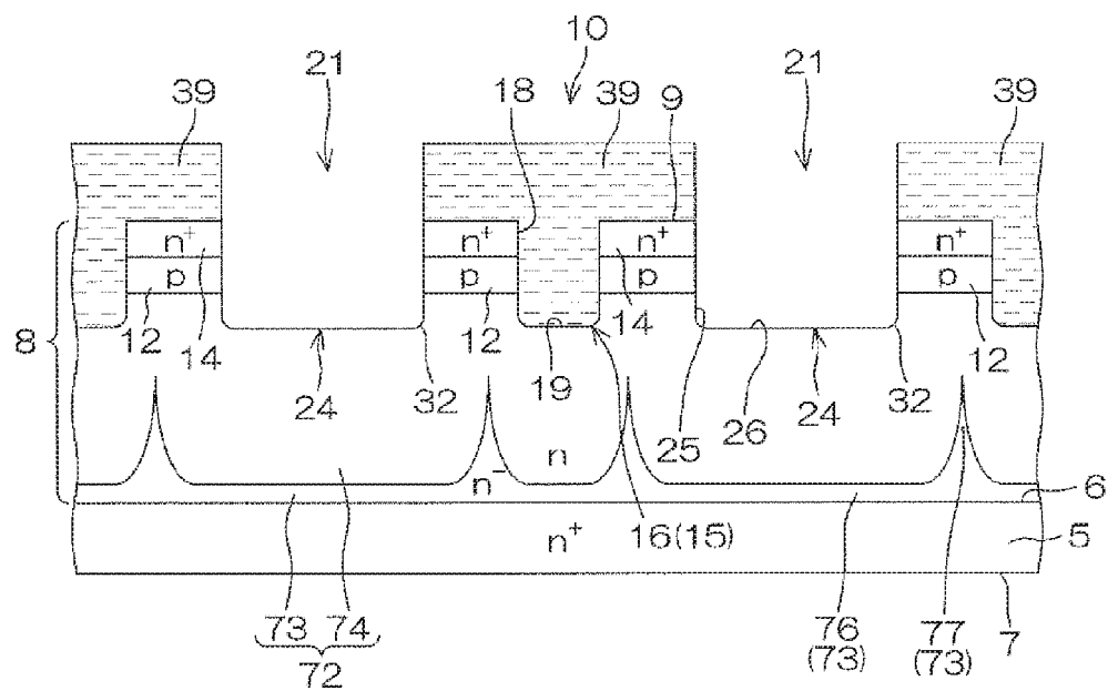
B-B SECTION
