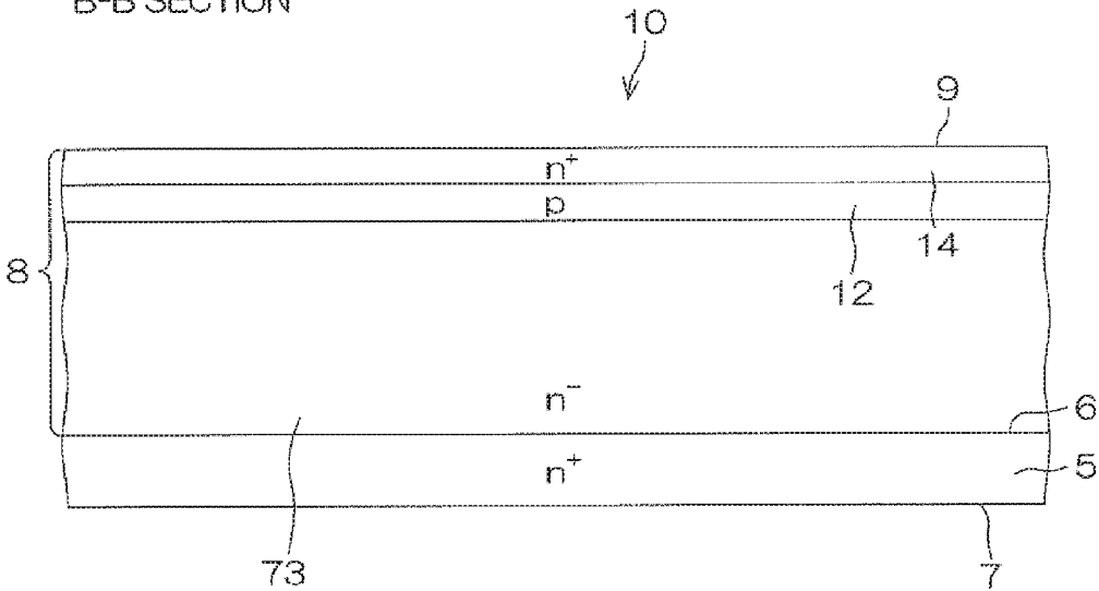
B-B SECTION
