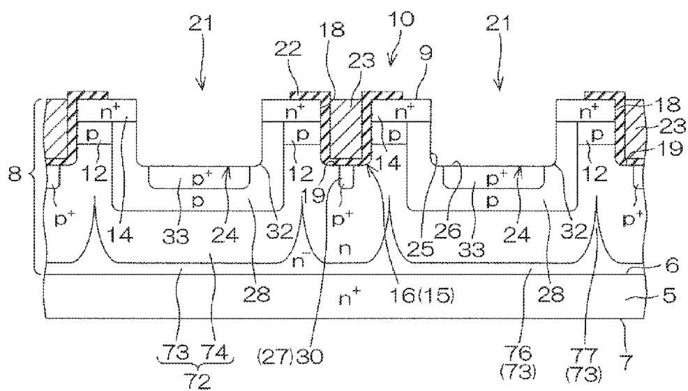
B-B SECTION
