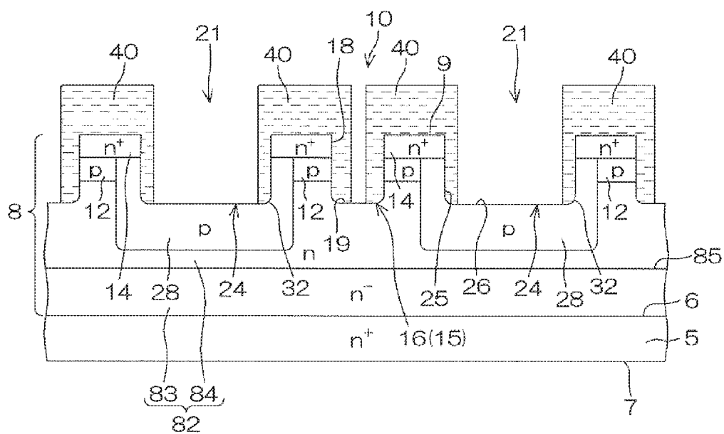
B-B SECTION
