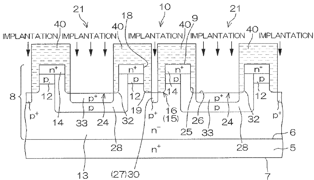
B-B SECTION
