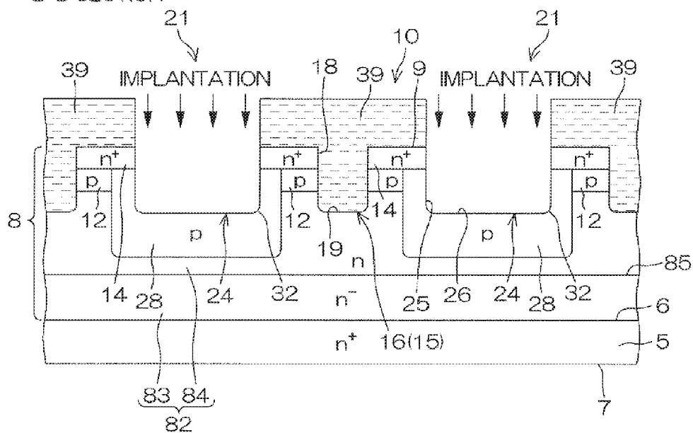
B-B SECTION
