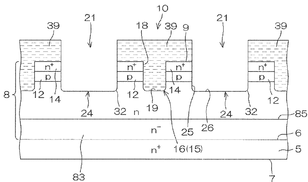
B-B SECTION
