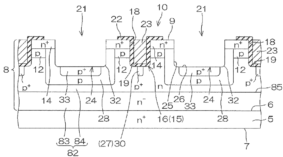
B-B SECTION
