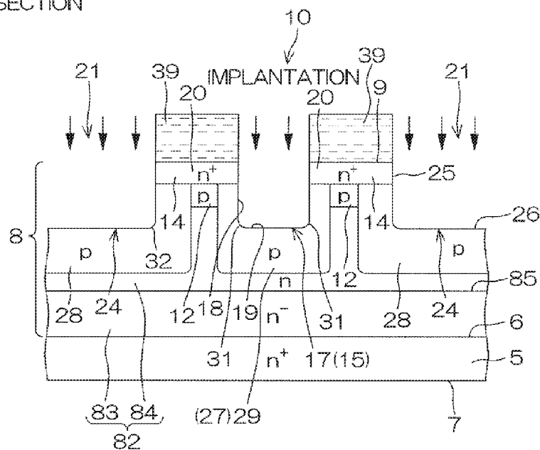
FIG. 11D A-A SECTION
