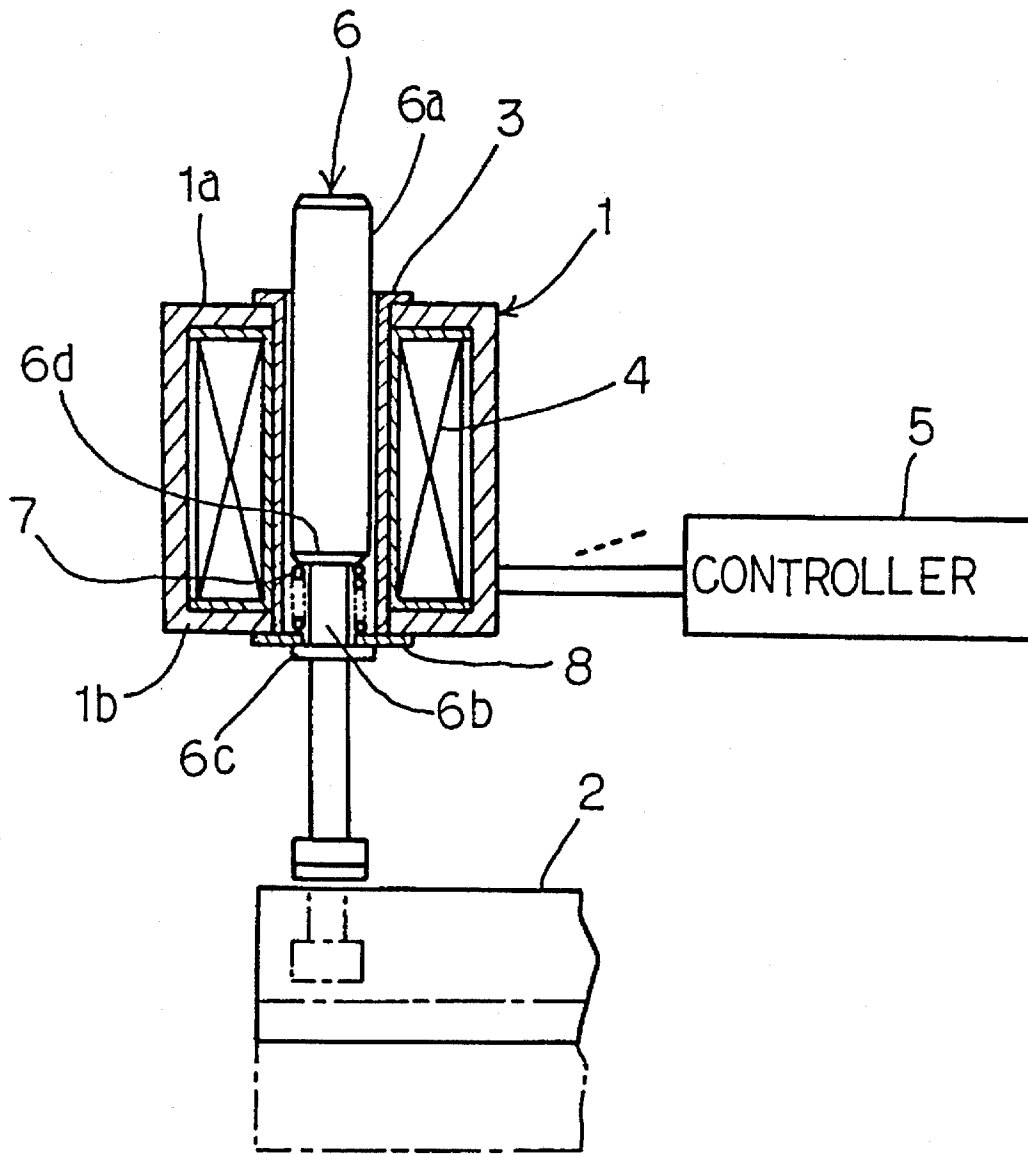
Fig. 1 PRIOR ART
