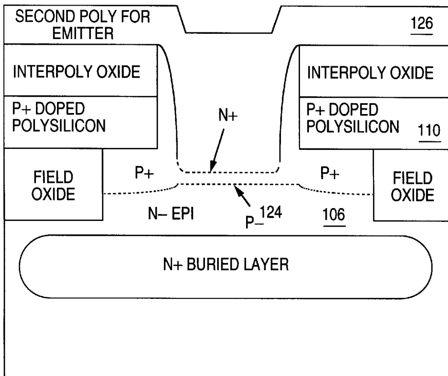
FIG. 1F (PRIOR ART)
