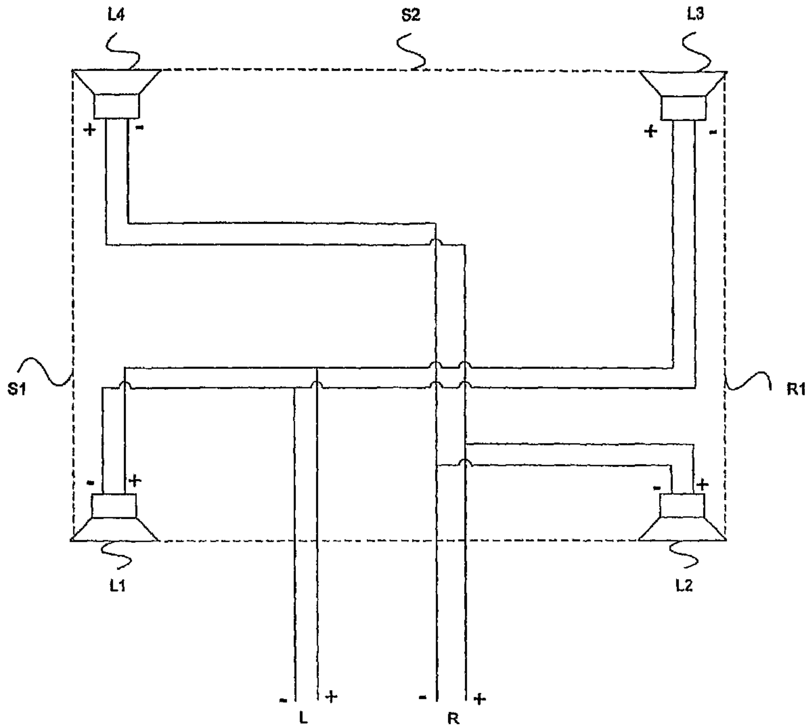
Input Signals
