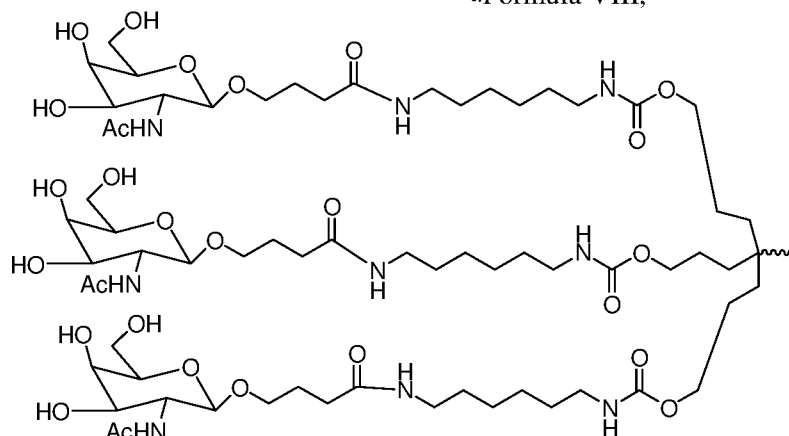
Formula VIII,
