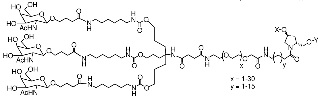
(Formula XXXIX),
