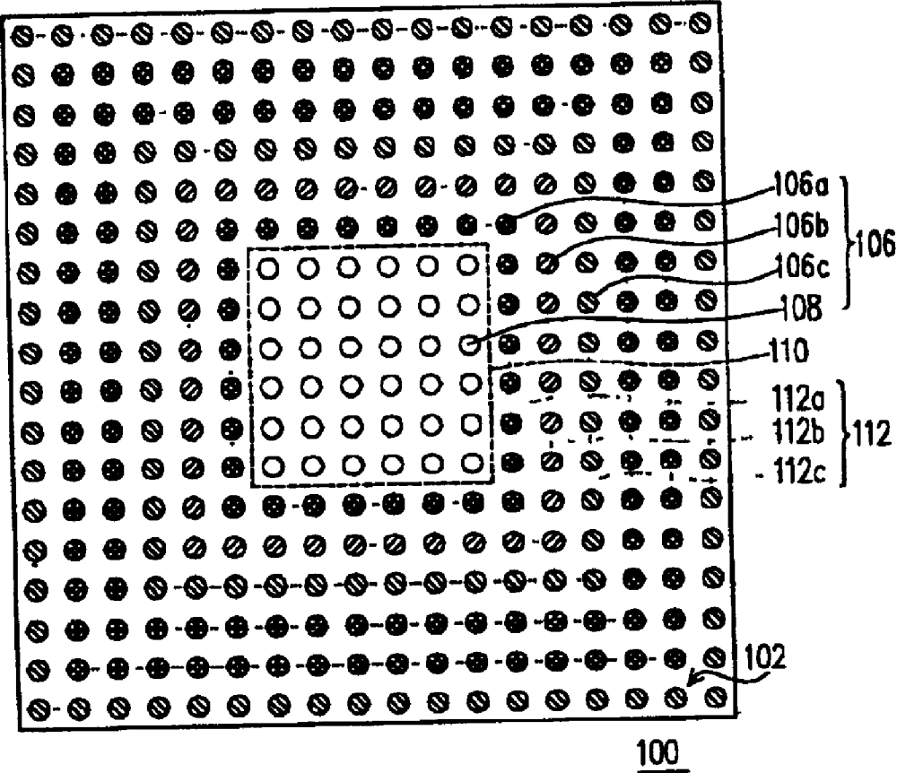
FIG. 2A(PRIOR ART)
