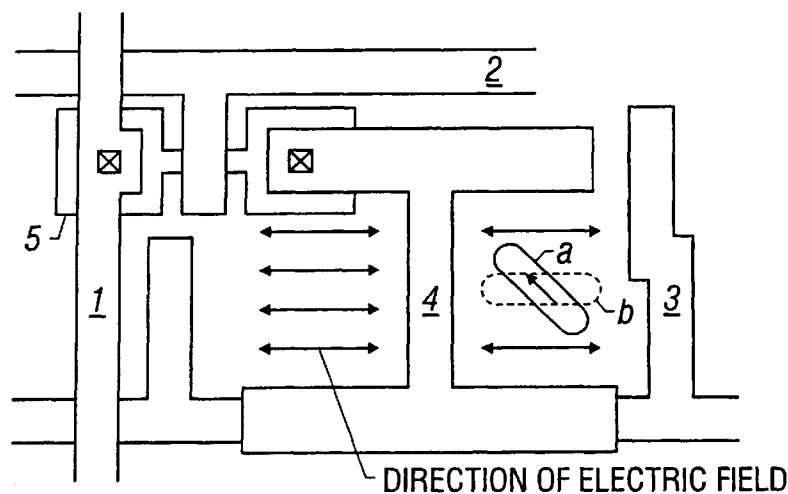
FIG. 7 (PRIOR ART)
