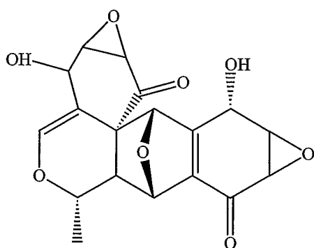
epoxyquinol A
