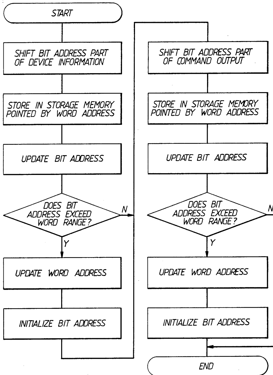
Fig. 3. PRIOR ART
