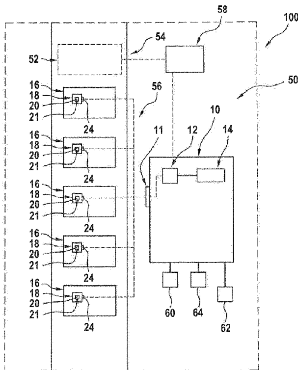
10 CONTROL UNIT 11 INTERFACE 12 CONTROLLER 14 MEMORY DEVICE 16 SHAFT DOOR 18 LOCKING DEVICE 20 SENSOR ELEMENT 21 SWITCH 24 SAFETY SWITCH 50 ELEVATOR-MONITORING APPARATUS 52 CAR 54 ELEVATOR SHAFT 56 SAFETY CHAIN 58 DRIVE 60 MAINTENANCE SWITCH 62 SIGNAL GENERATOR 64 DEVICE FOR STORING/RESETTING THE REFERENCE SEQUENCE 100 ELEVATOR INSTALLATION
