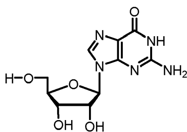
guanosine
