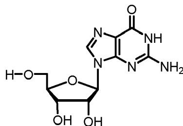
guanosine
