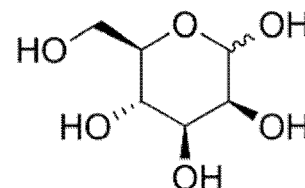
D-mannose
