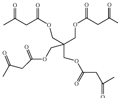
2,2-bis(((3-oxobutanoyl)oxy)methyl)propane-1,3-diyl bis(3-oxobutanoate)
