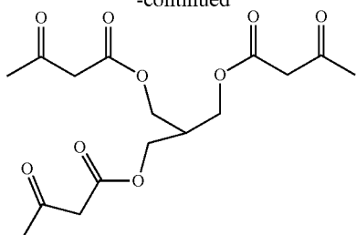
2-(((3-oxobutanoyl)oxy)methyl)propane-1,3-diyl bis(3-oxobutanoate)
