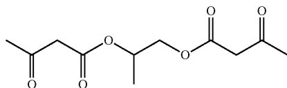
propane-1,2-diyl bis(3-oxobutanoate)
