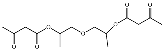
oxybis(propane-1,2-diyl) bis(3-oxobutanoate) & isomers
