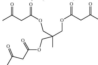
2-methyl-2-(((3-oxobutanoyl)oxy)methyl)propane-1,3-diyl bis(3-oxobutanoate)
