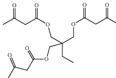
2-ethyl-2-(((3-oxobutanoyl)oxy)methyl)propane-1,3-diyl bis(3-oxobutanoate)
