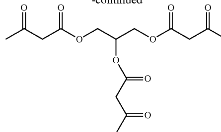
propane-1,2,3-triyl tris(3-oxobutanoate)
