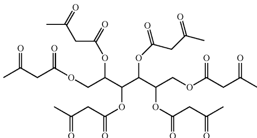
hexane-1,2,3,4,5,6-hexakis(3-oxobutanoate)
