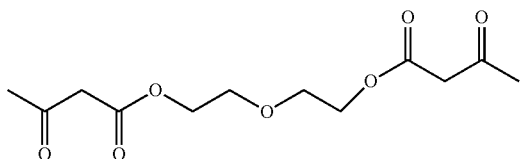
oxybis(ethane-2-1-diyl) bis(3-oxobutanoate)
