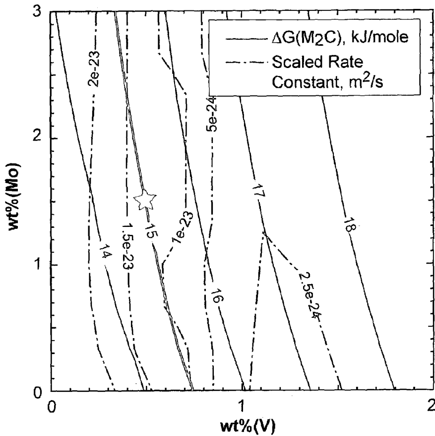
FIG. 4 CONTOURS OF M_2C DRIVING FORCE ( \Delta G ) AND SCALED RATE CONSTANT FOR VARYING MOLBDENUM ( M_o ) AND VANADIUM ( V ) CONTENTS, WHERE TEMPERATURE HAS BEEN SET TO 482°C, AND AMOUNTS OF OTHER ALLOYING ELEMENTS HAVE BEEN SET TO, BY WEIGHT, 0.14% C, 9% Cr, 13% Co, AND 4.8% Ni.
