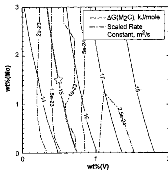
CONTOURS OF M_2C DRIVING FORCE ( \Delta G ) AND SCALED RATE CONSTANT FOR VARYING MOLYBDENUM (Mo) AND VANADIUM (V) CONTENTS, WHERE TEMPERATURE HAS BEEN SET TO 482°C, AND AMOUNTS OF OTHER ALLOYING ELEMENTS HAVE BEEN SET TO, BY WEIGHT, 0.14% C, 9% Cr, 13% Co, AND 4.8% Ni.
