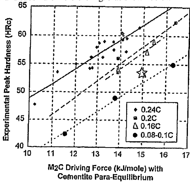
FIG. 3 CORRELATION BETWEEN PEAK HARDNESS AND M 2 C DRIVING FORCES FOR VARYING CARBON (C) CONTENT.
