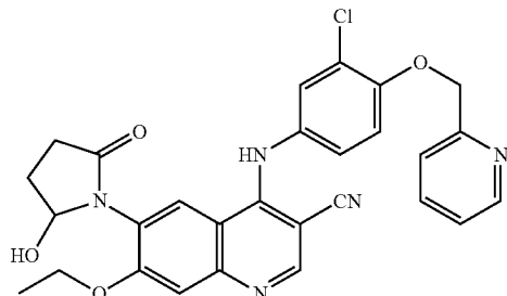
Degradation Product A
