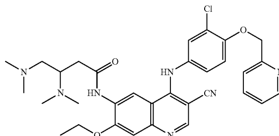
Process Impurity D
