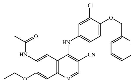
N-[4-[3-chloro-4-(2- pyridinylmethoxy)anilino]-3-cyano-7- ethoxy-6-quinolinyl]acetamide Exact Mass: 487.14
