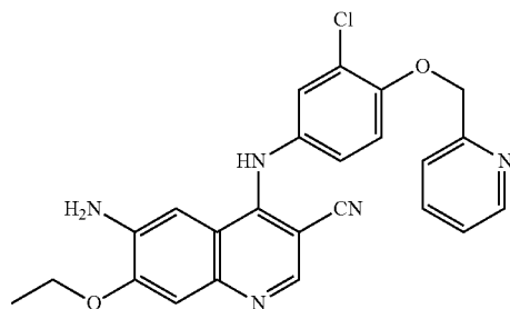
Process Impurity C
