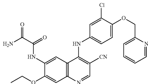
N¹-[4-[3-chloro-4-(2- pyridinylmethoxy)anilino]-3-cyano-7- ethoxy-6-quinolinyl]-ethanediamide Exact Mass: 516.13
