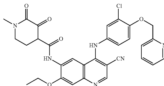
Process Impurity E
