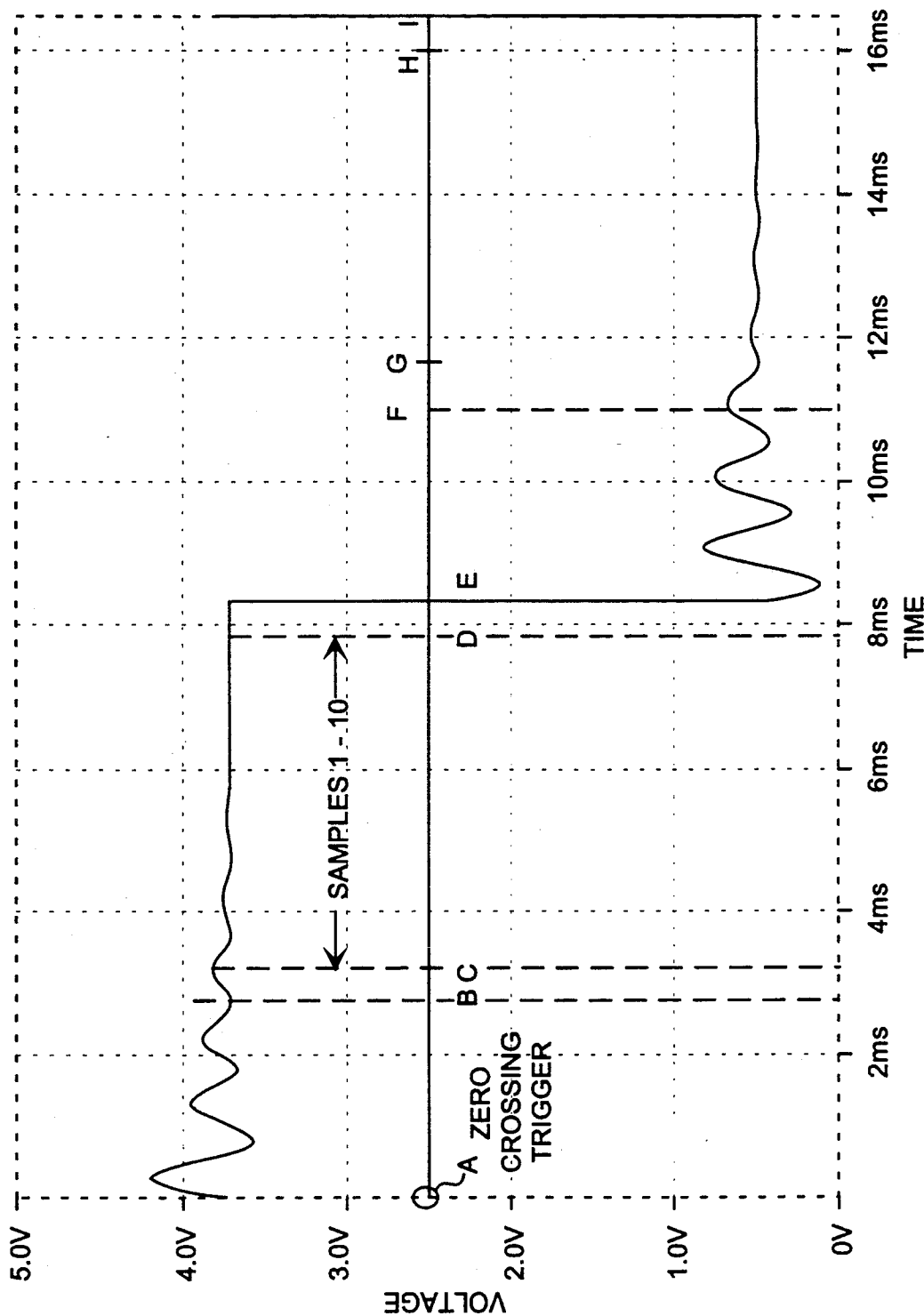
FIG. 4 (DETECTOR VOLTAGE)
