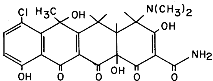
Dehydrochlortetracycline
