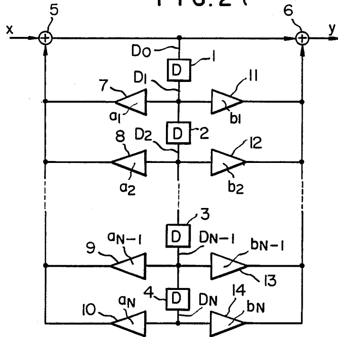
FIG. 2 (PRIOR ART)
