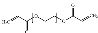
A9. Poly(ethylene glycol) diacrylate
