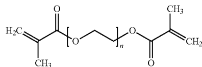
A11. Poly(ethylene glycol) methyl acrylate
