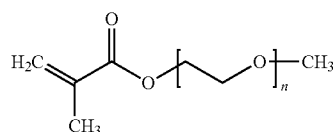
A12. Poly(ethylene glycol)methyl ether methacrylate
