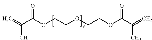
A7. Triethylene glycol dimethacrylate
